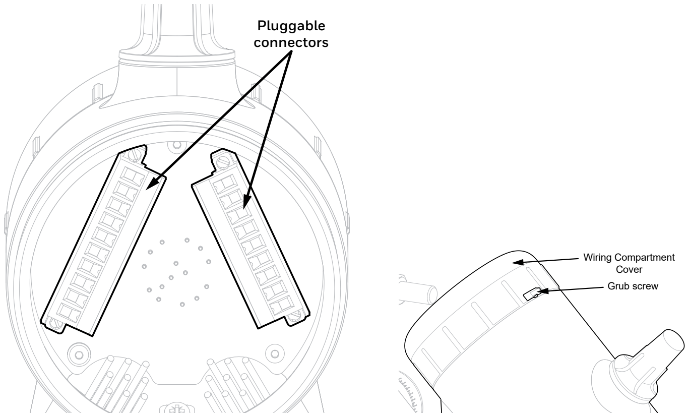
Figure 17. PCB Terminals
