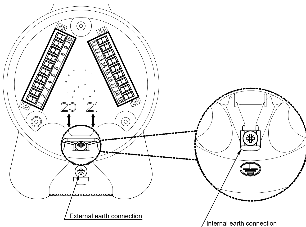
Figure 21. Terminal Wiring Compartment
