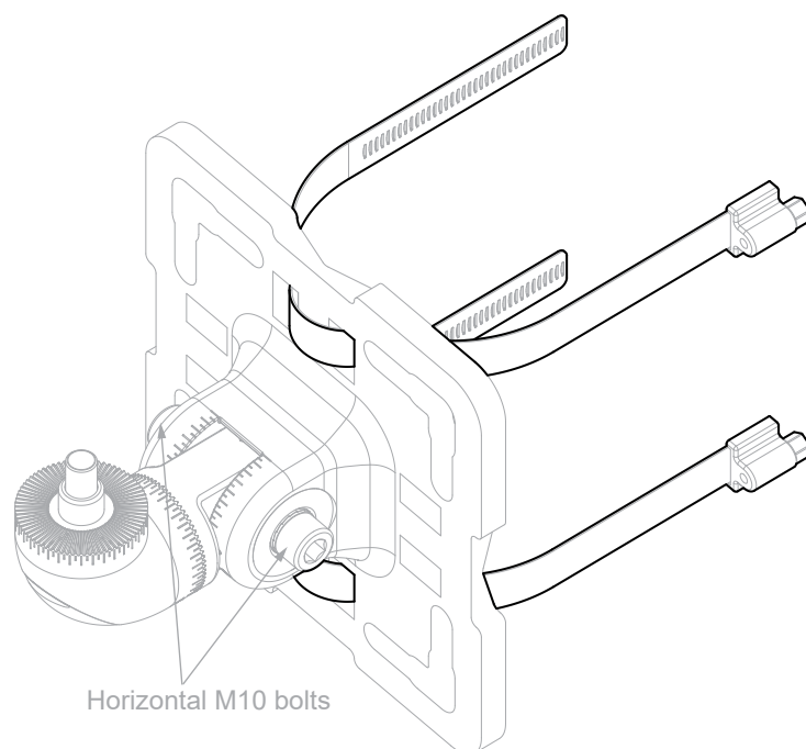
Figure 11. Universal Mounting Bracket fitment using Worm Drive Clips
