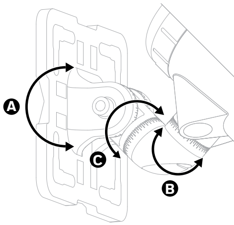
Figure 4. Adjustment ranges
